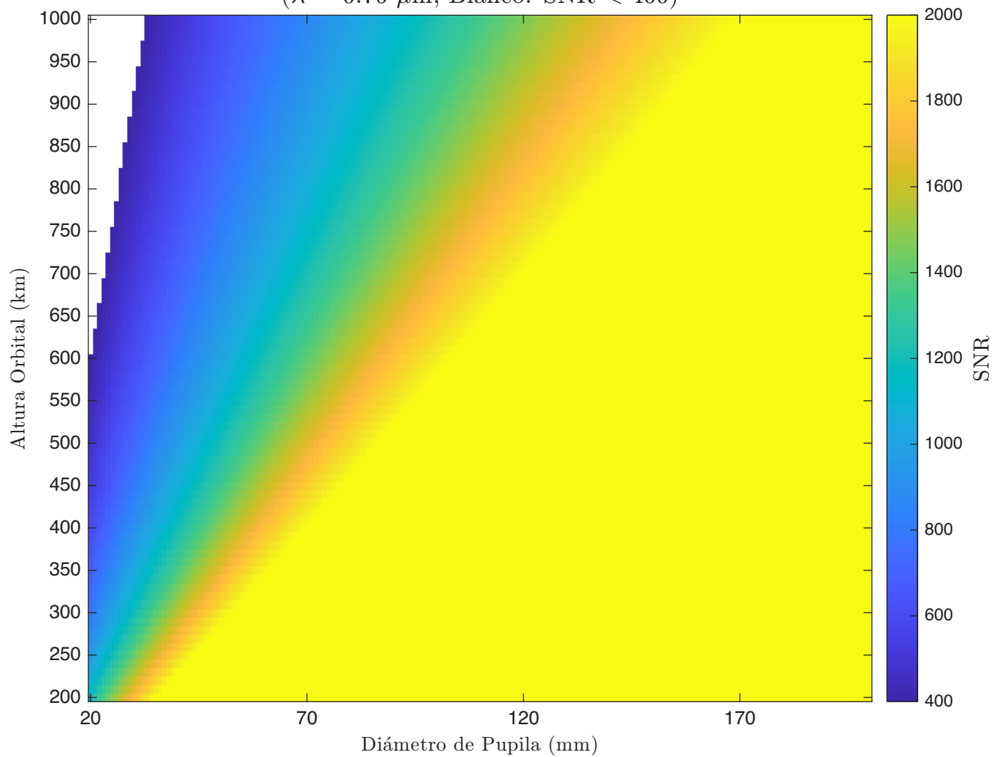
SNR - Cassegrain - Detector 2 ( \lambda = 0.76 \mu\text{m} , Blanco: \text{SNR} < 400 )
